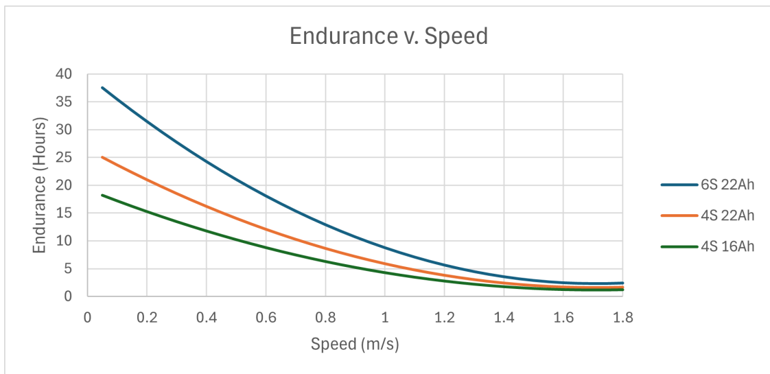
Figure 13: HyDrone™ ASV Endurance Chart
