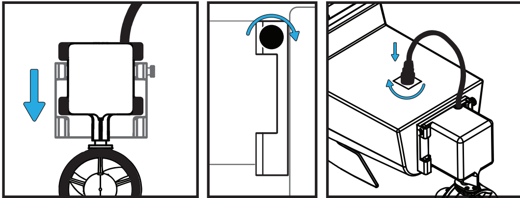
Figure 64: Thruster Installation
