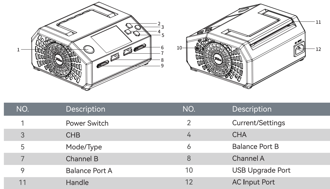
Figure 17: Tattu Charger Layout
