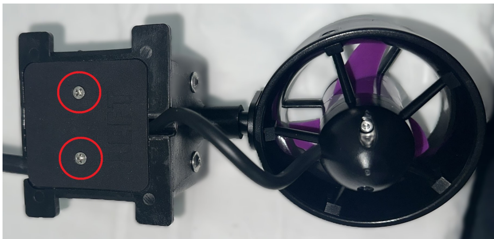
Figure 71: Servo Thruster Access Panel
