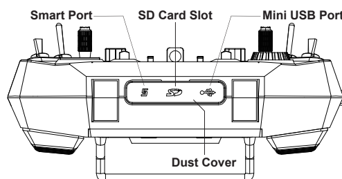
Figure 17: Bottom View
