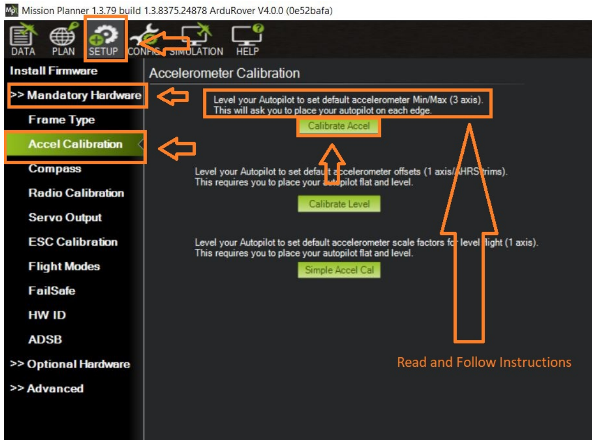
Figure 66: Accel Calibration Steps
