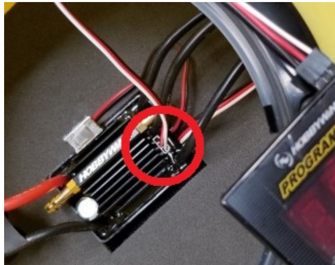
Figure 63: ESC Programming Card Connection
