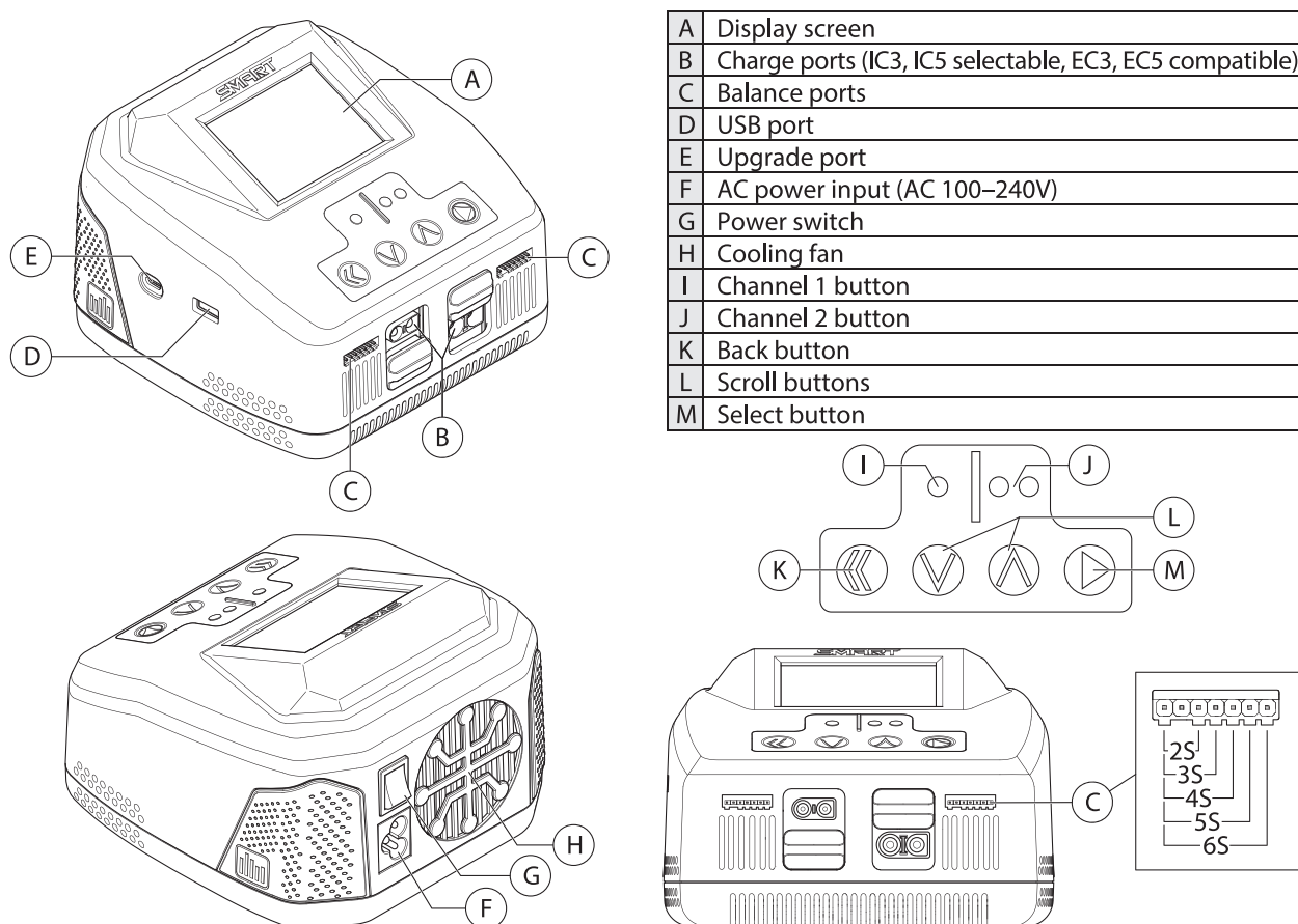
Figure 23: Spektrum Charger Layout
