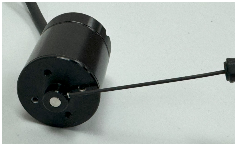
Figure 89: Rotor Removal
