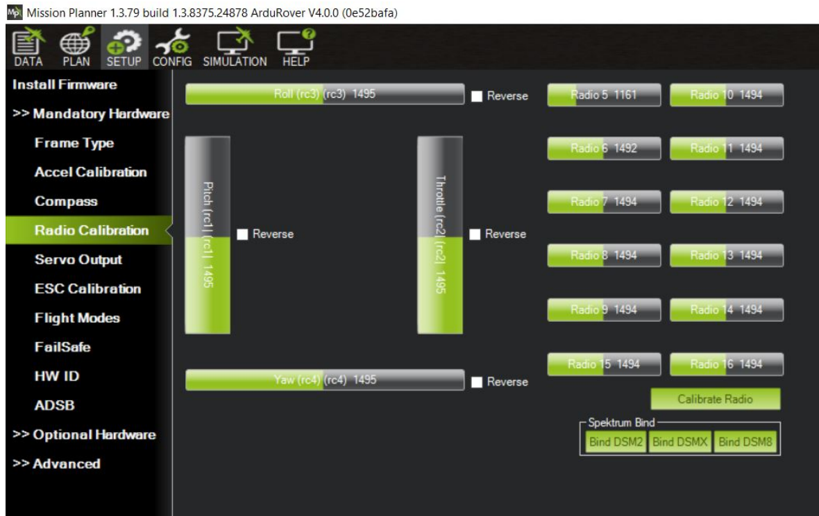
Figure 56: Setup Tab
