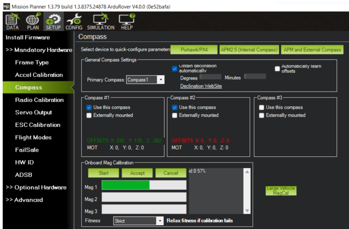
Figure 71: Compass Calibration Progress
