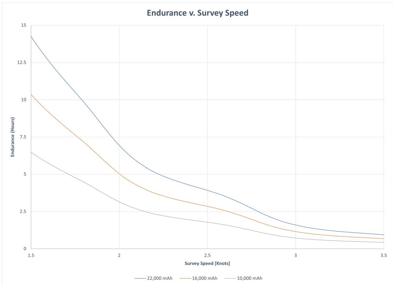
Figure 16: HyDrone™ ASV Endurance Chart
