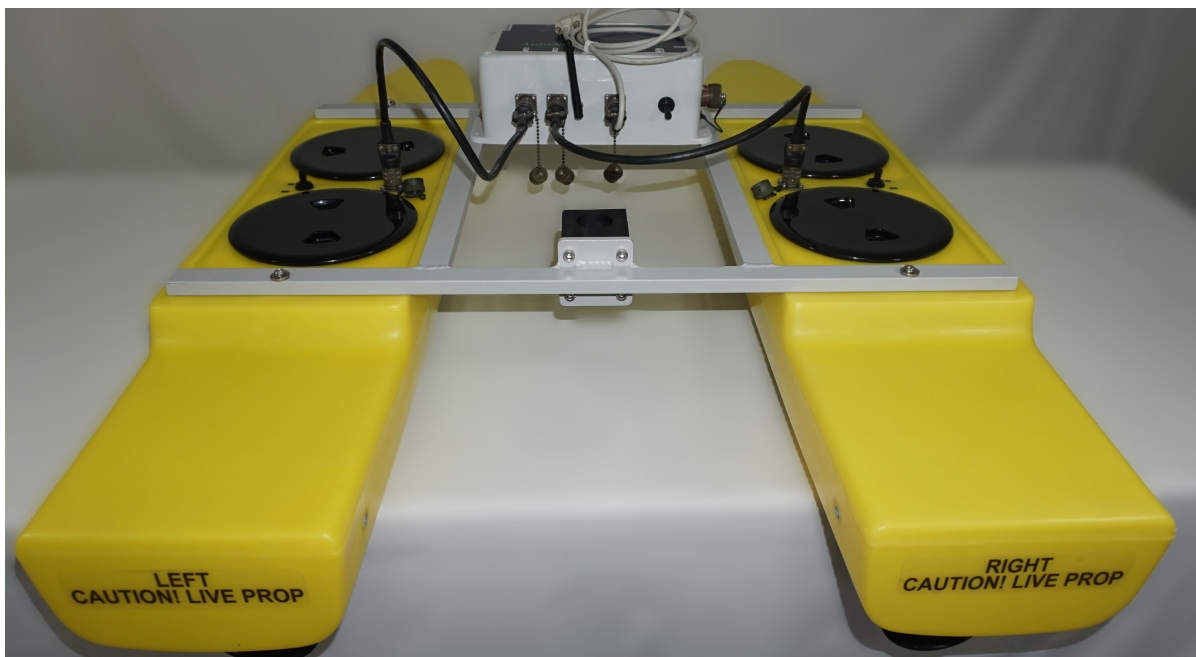
Figure 15: HyDrone™ ASV Assembled
